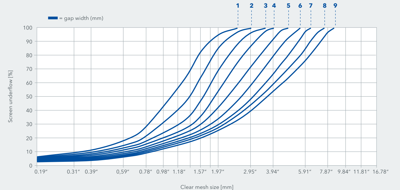
Crushing curve for the MOBICAT MC 100i EVO
